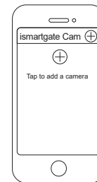
Tap "+" button
